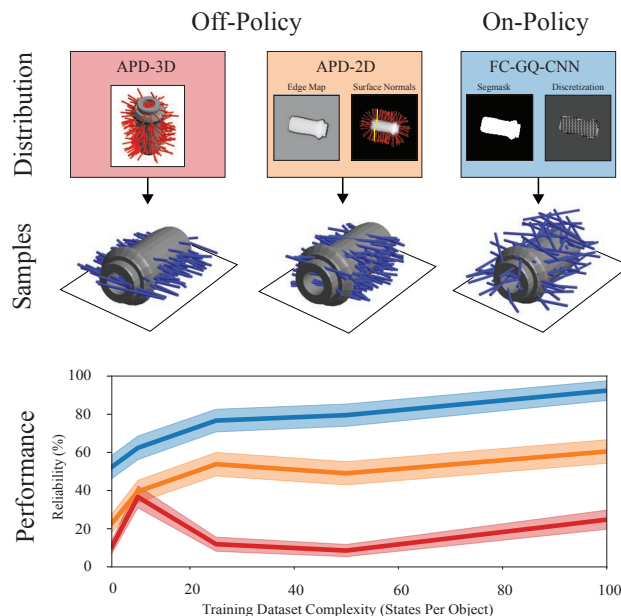
Fig. 1: Grasp action distributions for generating synthetic data to train robust grasping policies. (Top Left) 3D antipodal grasps sampled from object models (used by Dex-Net 2.0 [21]). (Top Middle) 2D antipodal grasps sampled from depth images. (Top Right) The proposed on-policy distribution where grasp actions are sampled from a 4-DOF dense discretization of actions based on a depth image and segmask. (Bottom) Performance in simulation on a singulated set of 10 objects with varying geometries of the FC-GQ-CNN policy trained on actions sampled from the off-policy APD-3D and APD-2D distributions and the on-policy FC-GQ-CNN distribution with supervisor guidance. The guided on-policy approach is able to reach performance close to that of a supervisor with full state knowledge.
